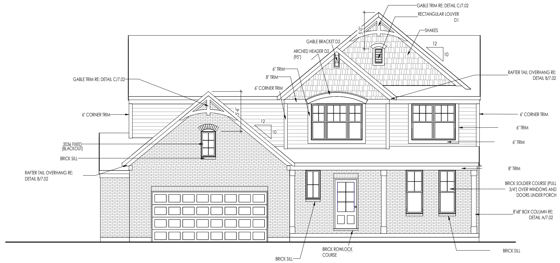
ELEVATION "D"
